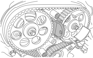
Locking the camshafts with KL-0482-301.
