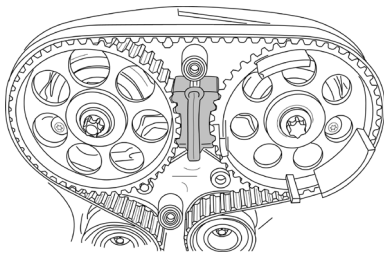
Locking the camshafts with KL-0482-302.
